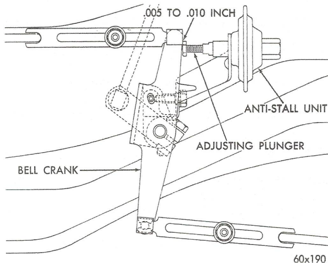
Fig. 16 Anti-Stall Adjustment
