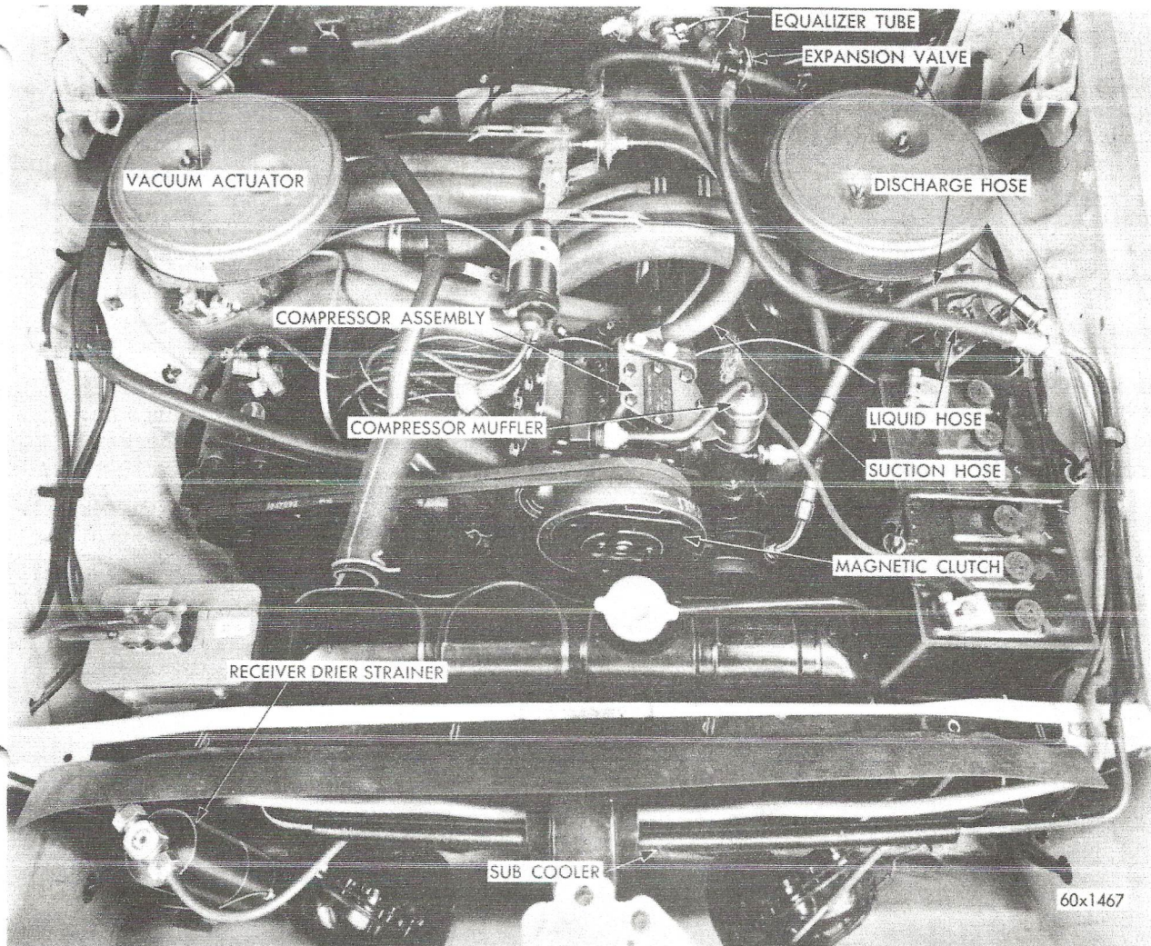
Fig. 19 Air Conditioning System Installed
