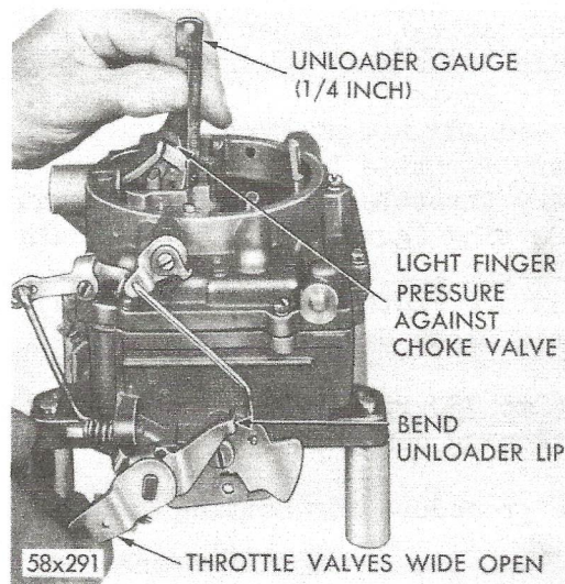
Fig. 8 - Checking and Adjusting Choke Unloader (Fast Idle Kick)
